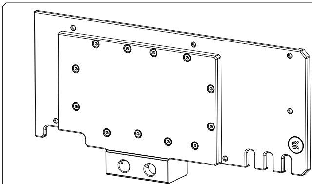
EK-Quantum Vector TRIO RTX 3080/3090 Active Backplate
